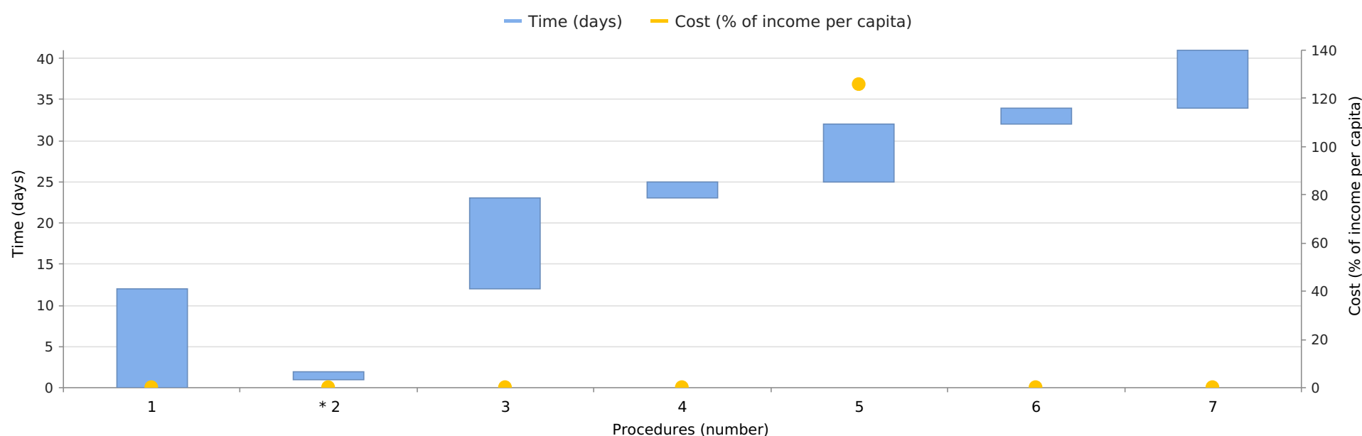
Figure - Getting Electricity in Azerbaijan - Procedure, Time and Cost
